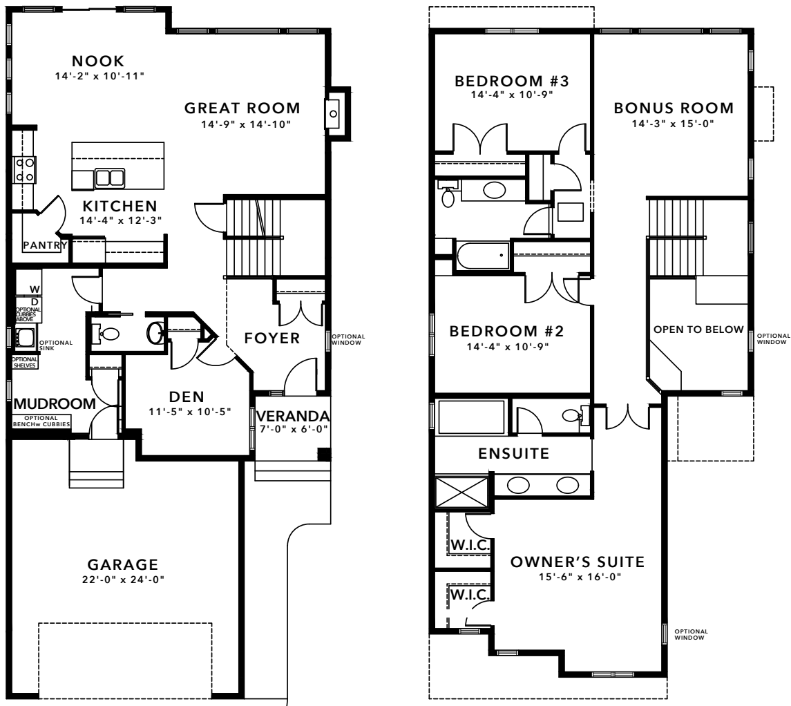
MAIN FLOOR 1165 sqft
