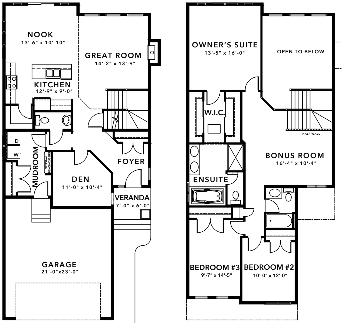
MAIN FLOOR 1019 sqft
